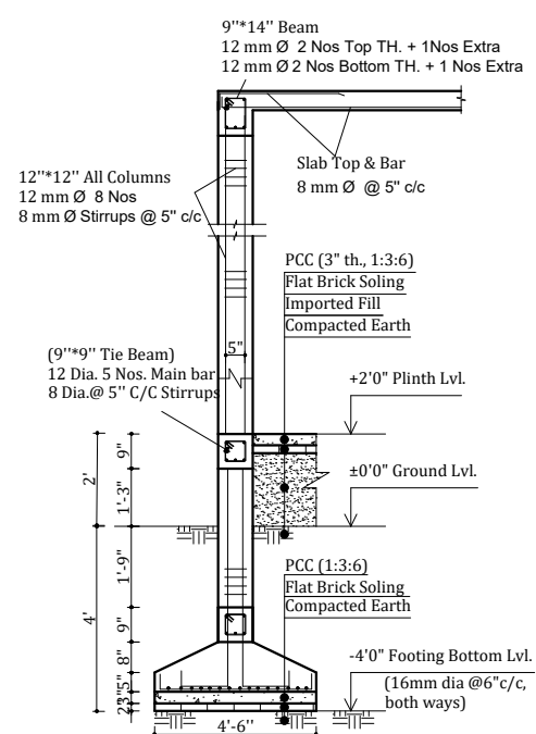
FIG: TYPICAL DETAILS FOR RCC STRUCTURE (SCALE=(1/4)"=1'-0")
