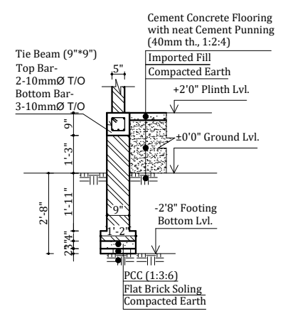
FIG: DWARF WALL FOOTING, FLOORING SECTION (SCALE: (1/4)"=1'-0")
