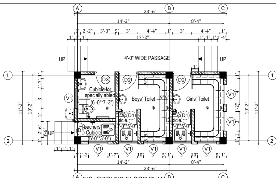
FIG: GROUND FLOOR PLAN (AREA= 262.49 SQ.FT.)
