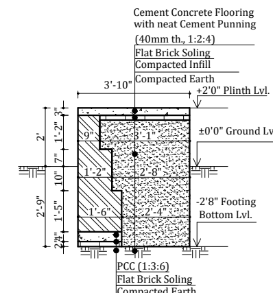
FIG: PASSAGE SECTION (SCALE: (1/4)"=1'-0")
