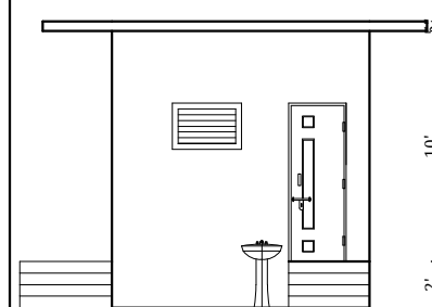
FIG: WEST ELEVATION
