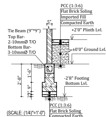
FIG: PARTITION WALL FOOTING, FLOORING SECTION (SCALE: (1/4)":1'-0")
