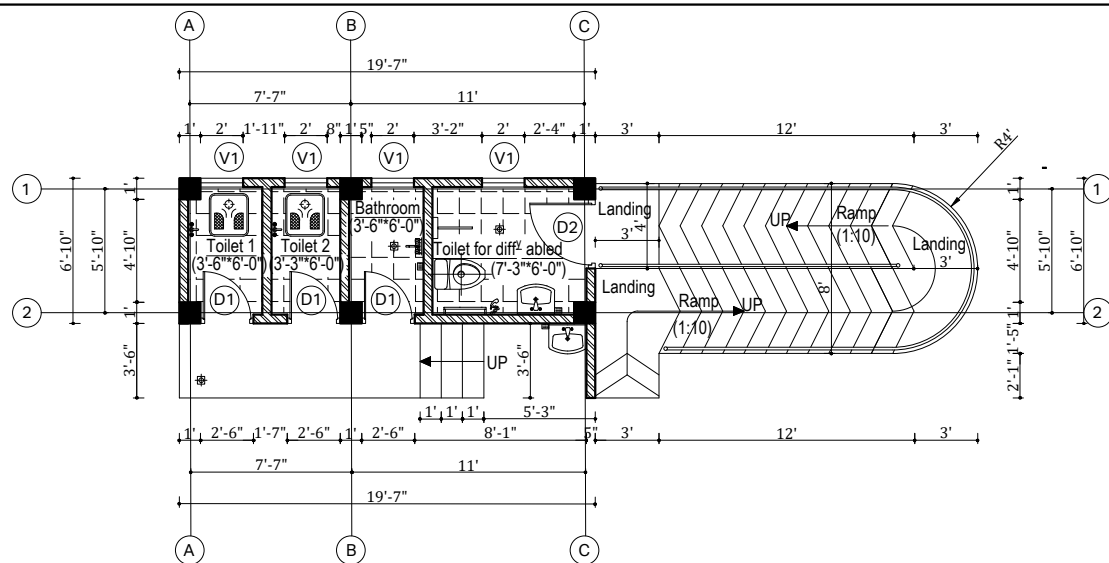
FIG: GROUND FLOOR PLAN (AREA= 133.73 SQ.FT.)
