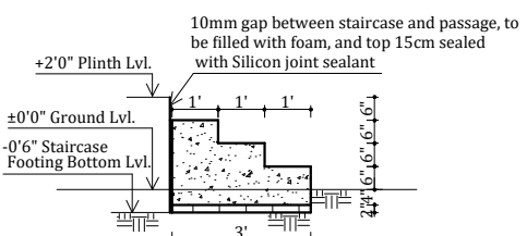
FIG: STEPS SECTION (SCALE: (1/4)":1'-0")
