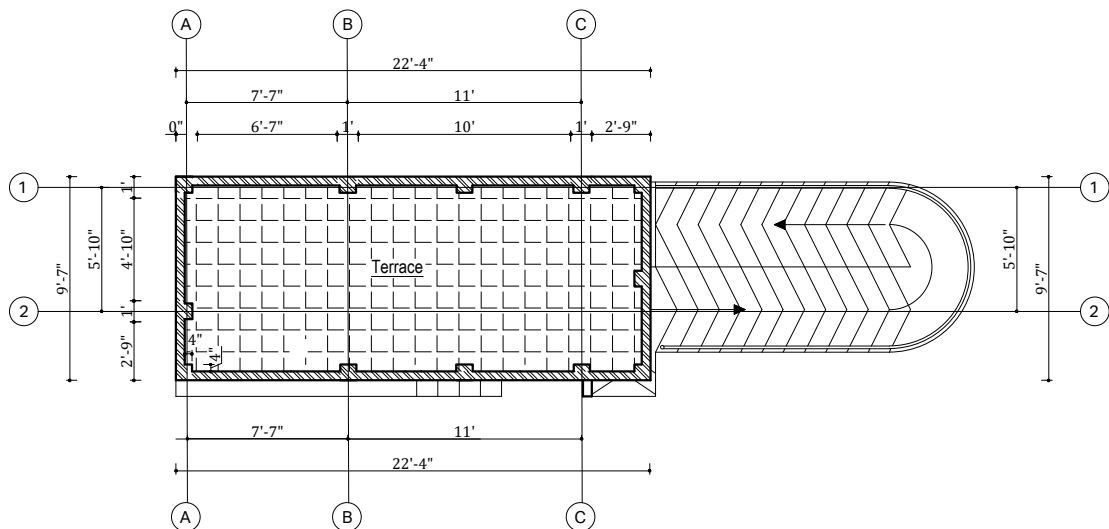
FIG: ROOF FLOOR PLAN
