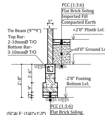
FIG: PARTITION WALL FOOTING, FLOORING SECTION
