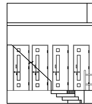
FIG: SOUTH ELEVATION
