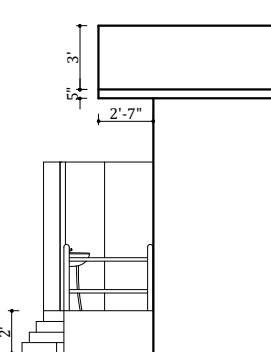
FIG: EAST ELEVATION
