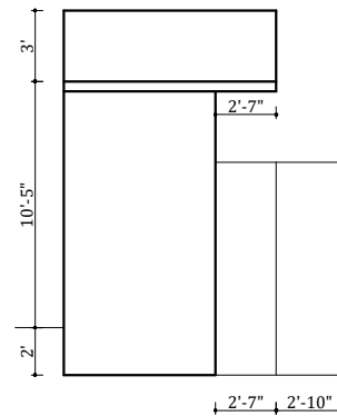
FIG: WEST ELEVATION
